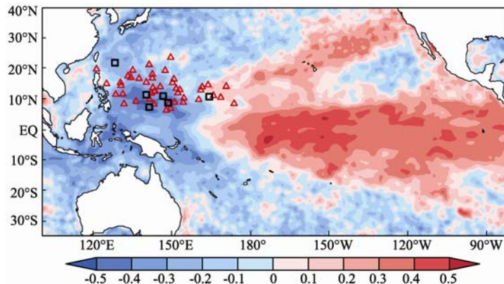
Fig.8 Correlation between STY Number and SSTA , the red triangles (black squares) denoting the formation locations of STYs in the maximal (minimal) STY number years.
