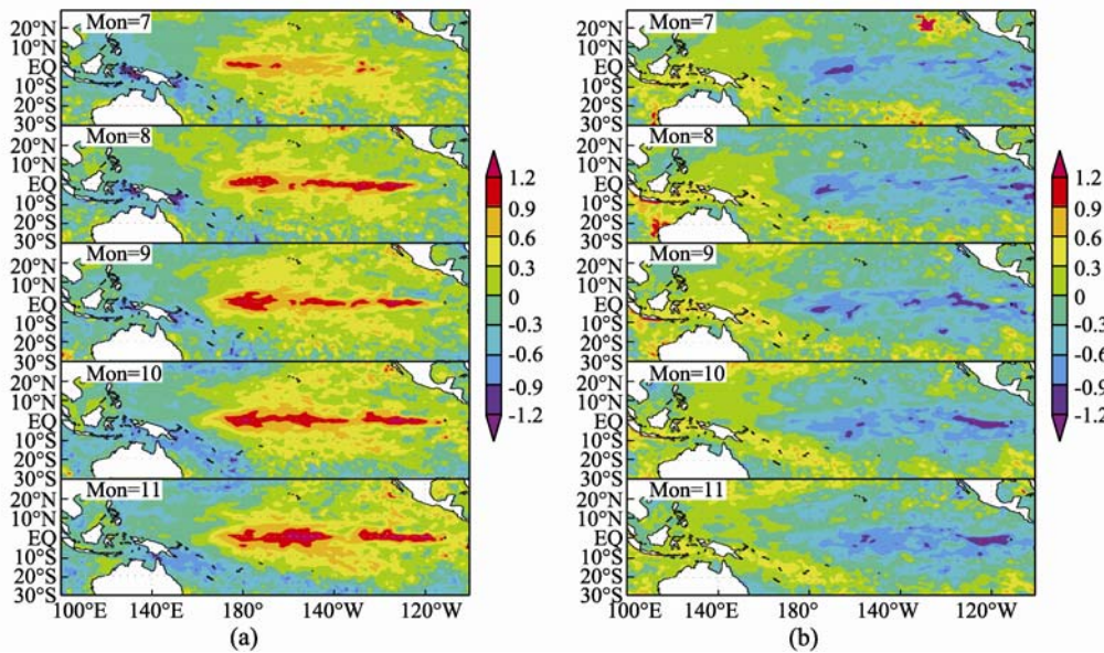
Fig.7 Composite SSTA fields from July to November for maximal and minimal STY number years.
