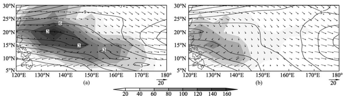
Fig.10 Vertical wind shear (200–850hPa) and frequency of STY in El Niño years (a) and La Niña years (b). The contours denote isotachs and shaded contours show the frequency of STY.
