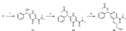
Scheme 3. Structural optimization of Unit C: Synthesis of compound 19 . Reagents and conditions: (I) dimethylamine in MeOH, 48 h, 80 °C; (II) AcOH, EDCl, DMAP, CH_2Cl_2 , 0 °C, 1 h; (III) 2-bromoethanol, K_2CO_3 , acetone, 48 h, 80 °C.
