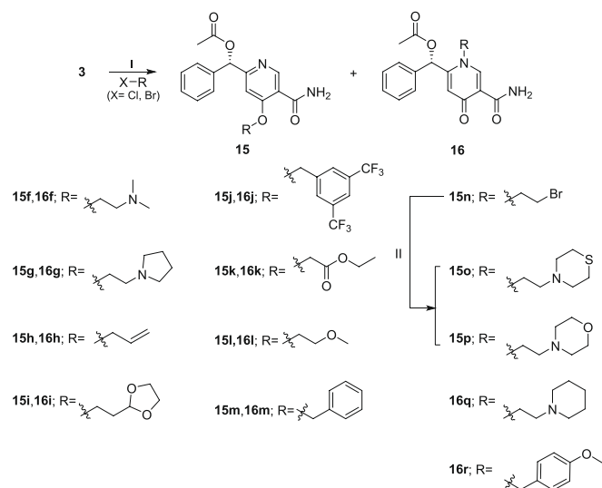
Scheme 2. Structural optimization of Unit B: Synthesis of compounds 15 and 16 . Reagents and conditions: (I) K_2CO_3 , acetone, 80 °C, overnight. (II) morpholine or thiomorpholine, K_2CO_3 , acetone, 80 °C, overnight.
